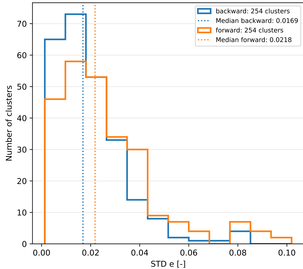
K=254 | Within-cluster STD distributions | Each cluster counts once
